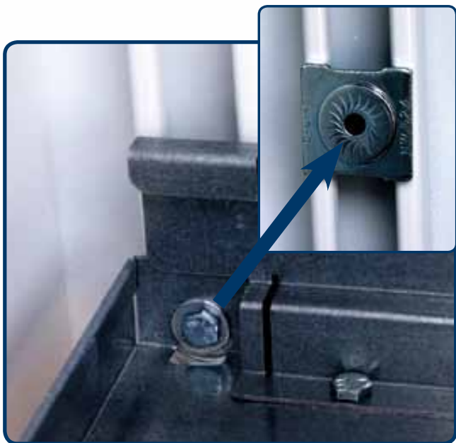
1/4-inch bolts hold FlexSmart components securely into adjustable channel clips
